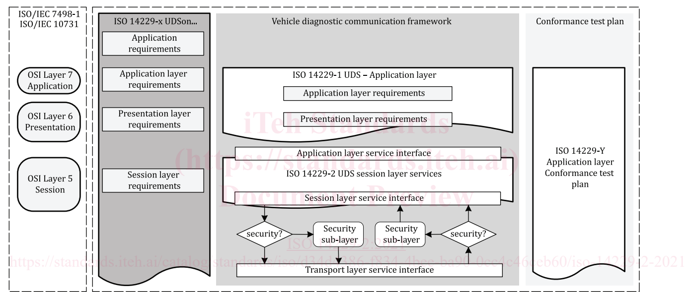
Figure 1 — ISO 14229 series reference according to OSI model
