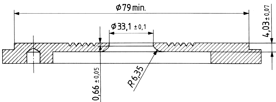
Figure 2 – Mâchoire inférieure alternative 1)
