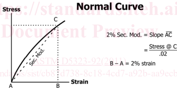
FIG. X1.1 Normal Curve
