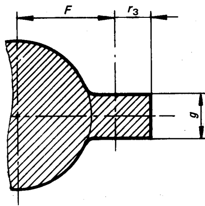
Drop forged hooks (Cross-section through tu)
