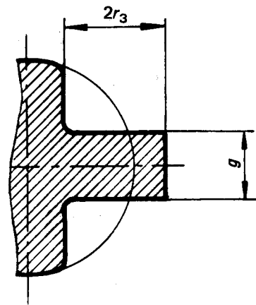
Hammer forged hooks (Cross-section through tu)
