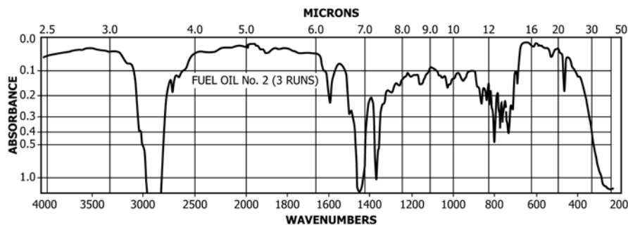
FIG. 1 Complete Spectrum of a No. 2 Fuel Oil, Analyzed in Triplicate
