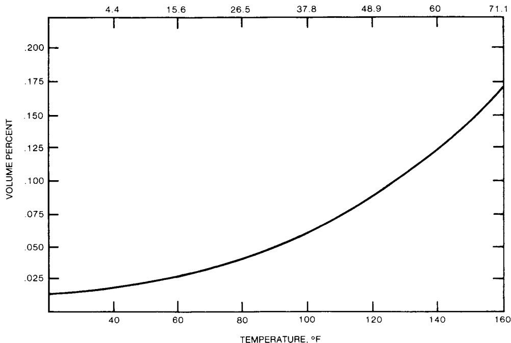
FIG. A1.1 Solubility of Water in Toluene
