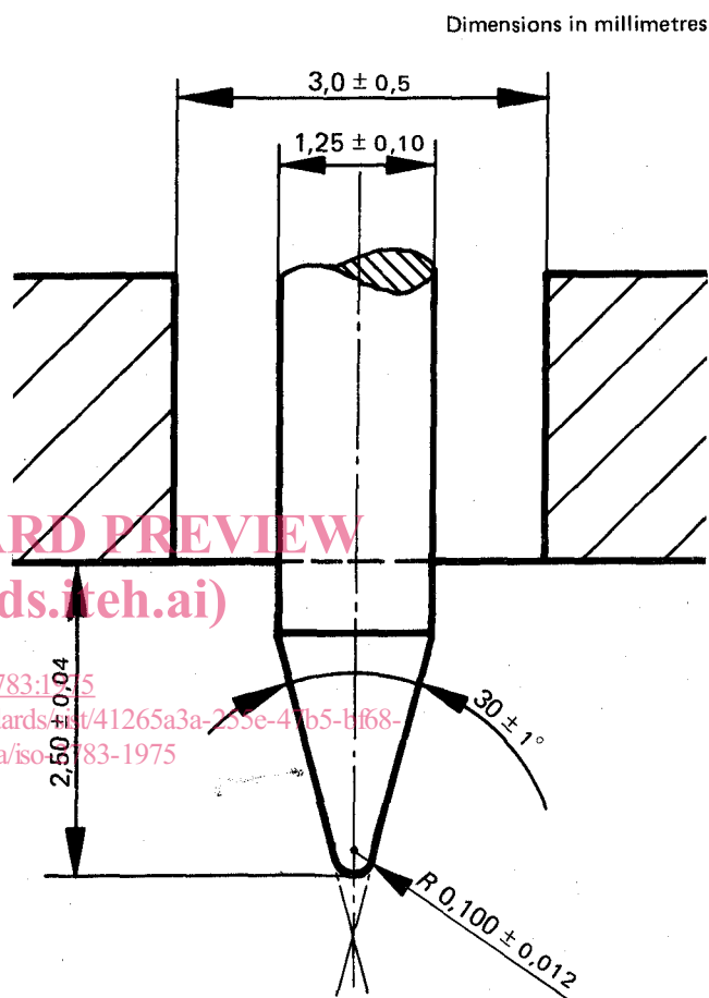
FIGURE 1 — Durometer indenter
