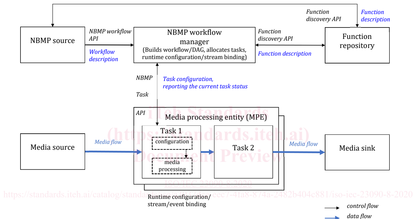
Figure 1 — NBMP reference architecture
