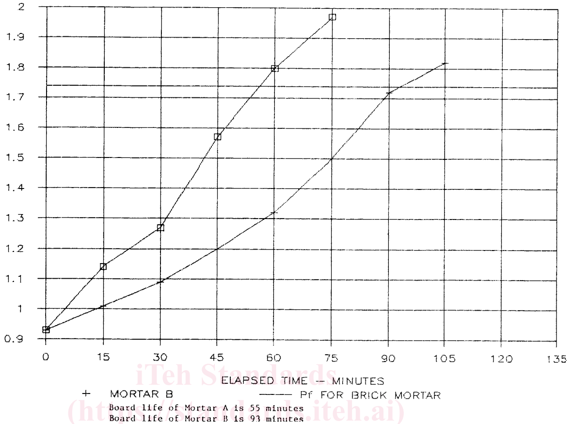
FIG. A3.1 Penetration Resistance Versus Elapsed Time
