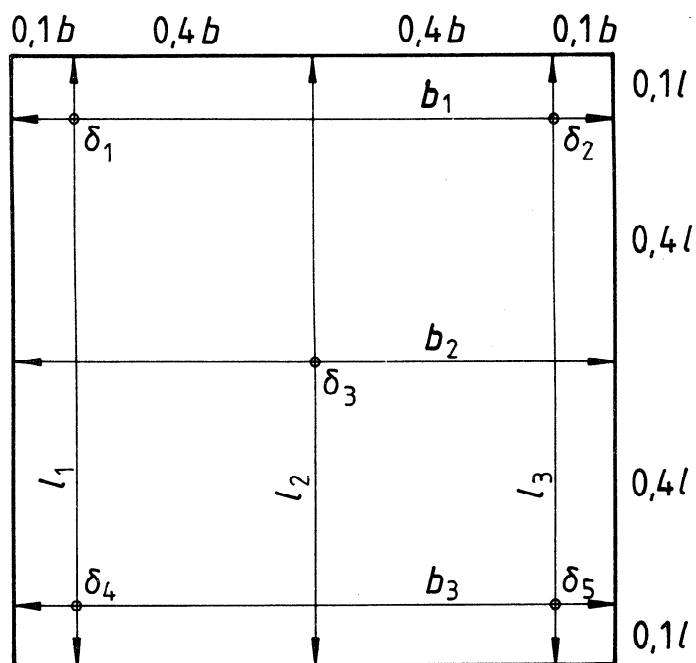
Figure Positions for measuring dimensions (standards.iteh.ai)
