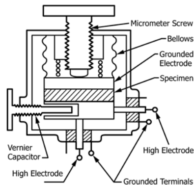
FIG. 10 Micrometer-Electrode System
