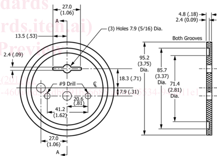
FIG. 2 Beaker Cover
