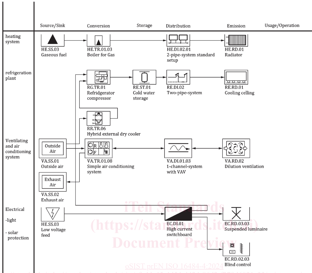
Figure 1 — Example for documentation of design choices for technical infrastructure of a building (Source: SN 502411:2016 / SIA 411:2016)
