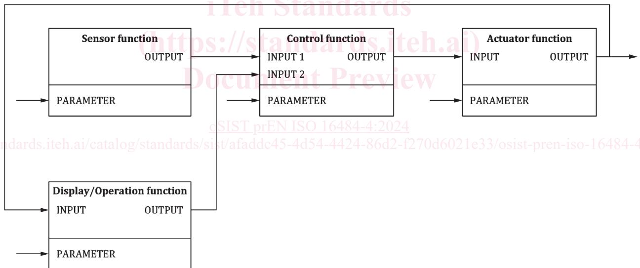
Figure 4 — Relationship between Automation functions (typical example)
