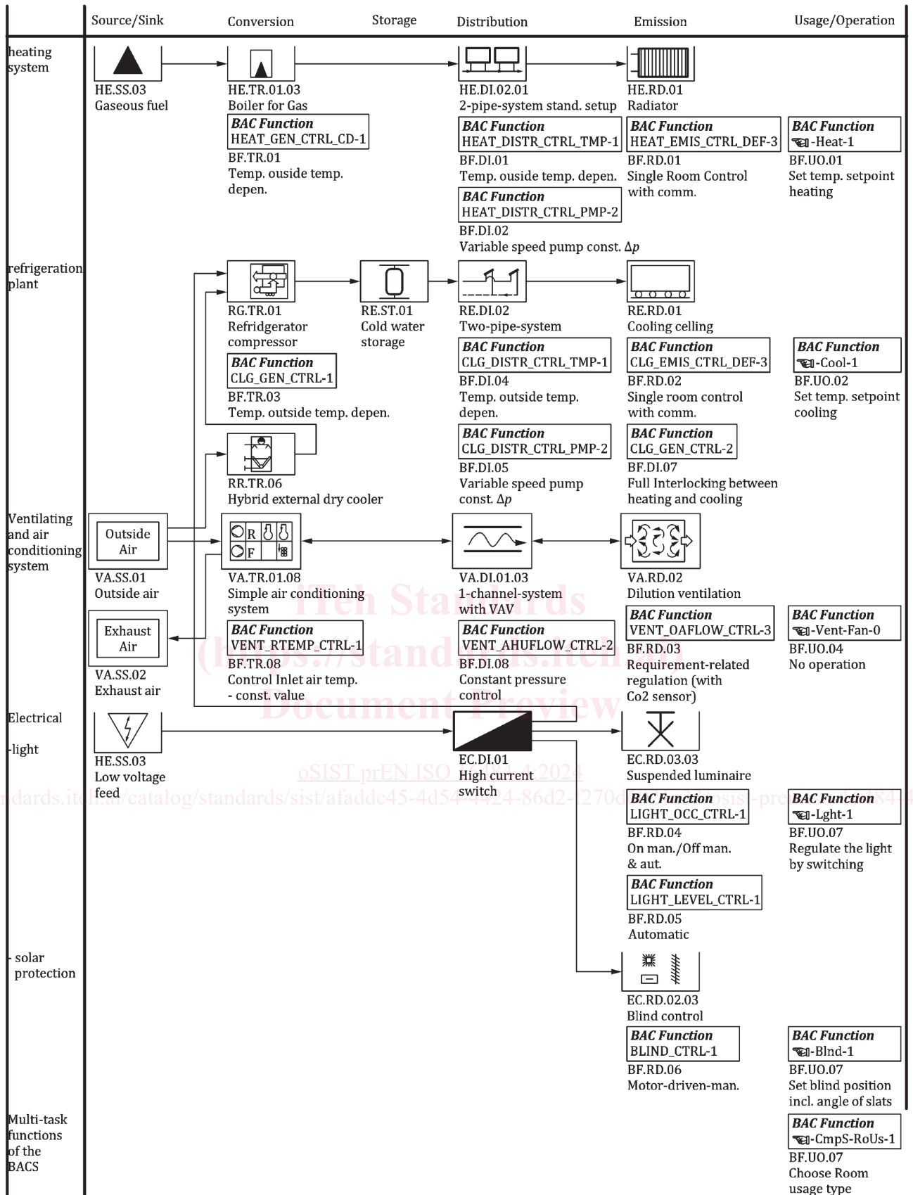
Figure 2 — Example for documentation of design choices for technical infrastructure and associated control functions of a building (Source: SN 502411:2016 / SIA 411:2016)
