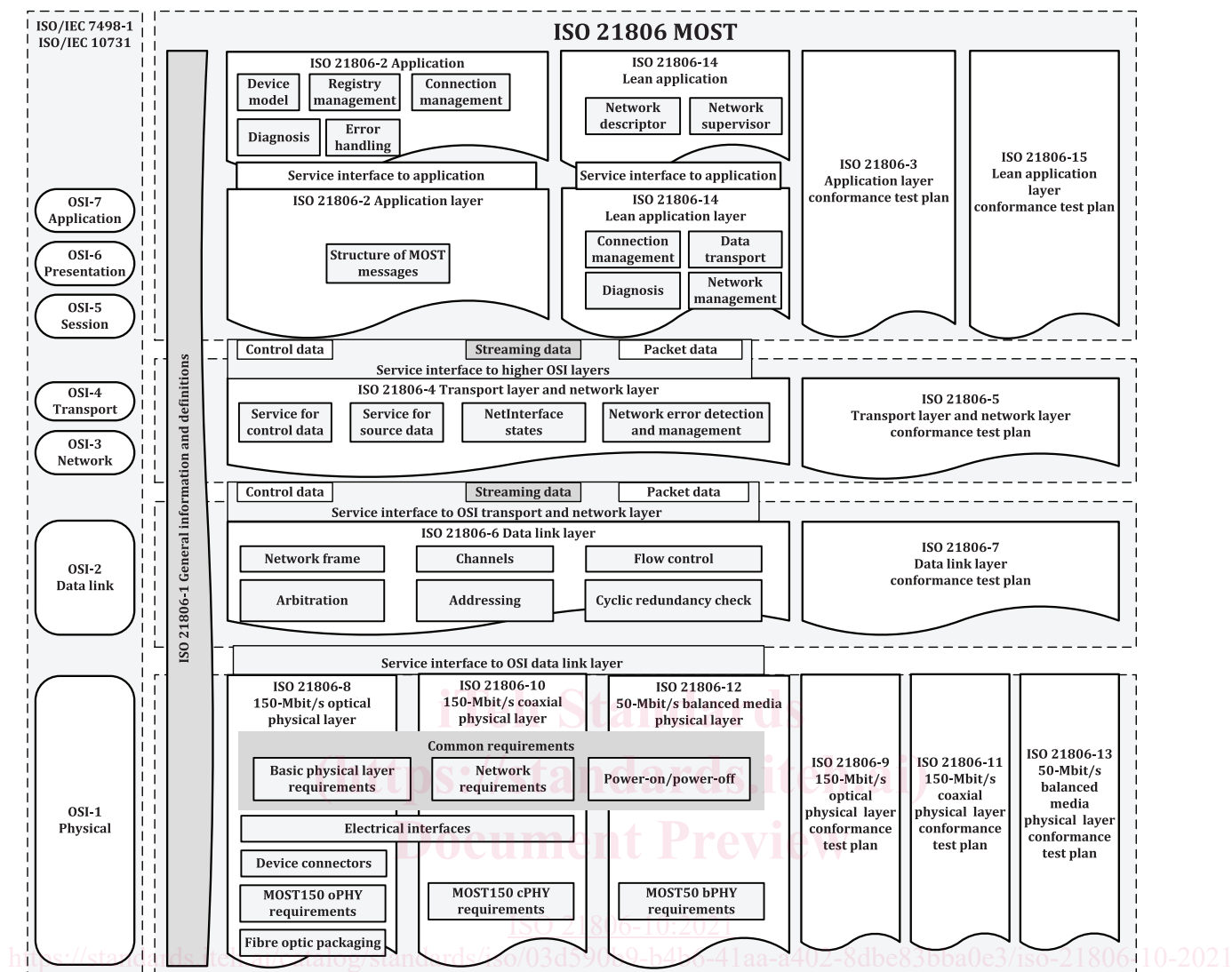
Figure 2 — The ISO 21806 series reference according to the OSI model
