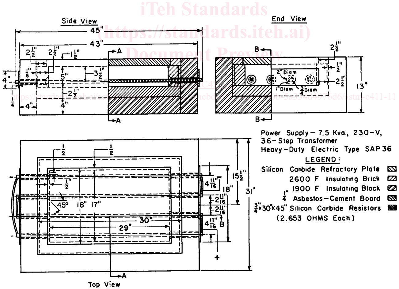
FIG. 1 Type A Heating Plate for Hot-Surface Performance Test
