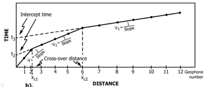
FIG. 5 (a) Seismic Raypaths and (b) Time-Distance Plot for a Three-Layer Model With Parallel Boundaries (4)
