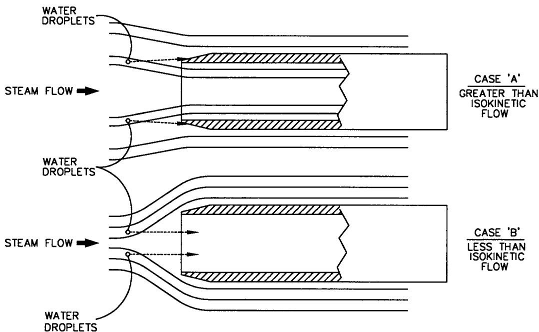
FIG. 1 Effect of None-Isokinetic Sampling
