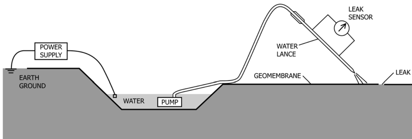
FIG. 1 Diagram of the Electrical Leak Location Method for Surveys with Water Lance on Exposed Geomembrane
