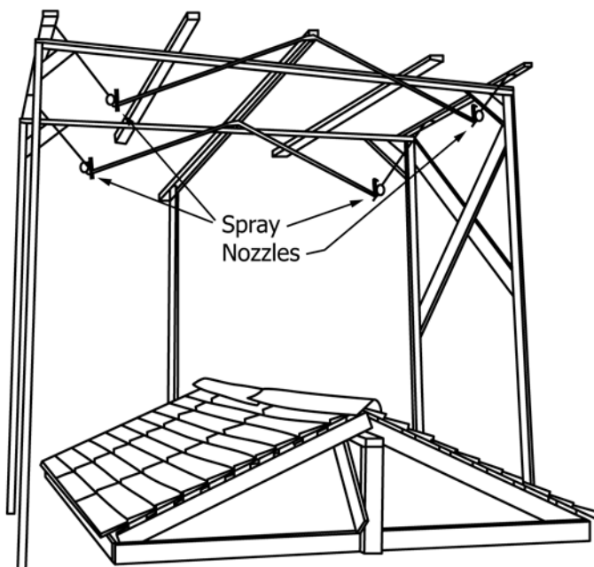
FIG. 1 Schematic Drawing of Fire Test Apparatus
