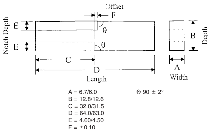
FIG. X1.2.1 Dimensions of Double-Notched Izod Test Specimens
