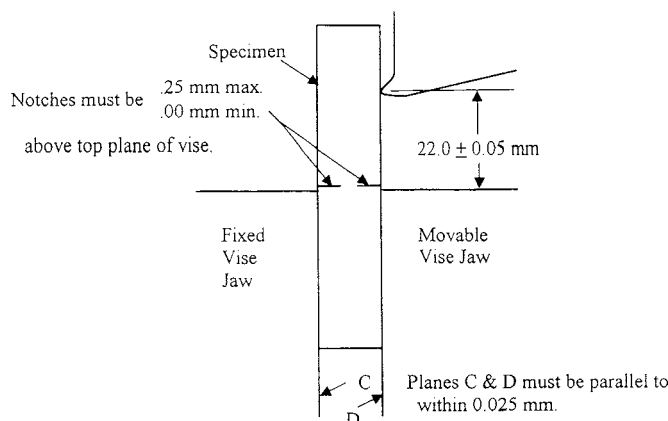
FIG. X1.2 Relationship of Vise, Specimen, and Strike Edge to One Another
