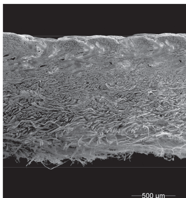
Figure A.2 — Typical section of sheep leather
