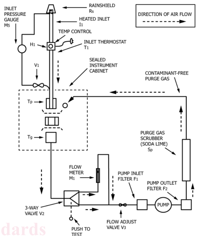
FIG. 1 Dual Tape Sampler Flow Schematic
