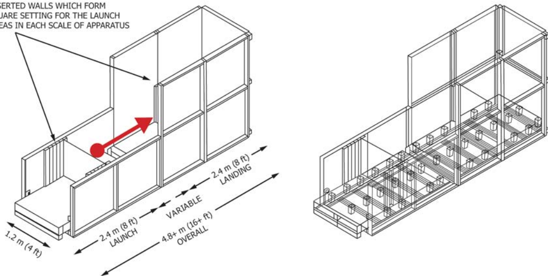
FIG. 2 Mobility: Confined Area Obstacles: Gaps Apparatus (Perspective Views)
