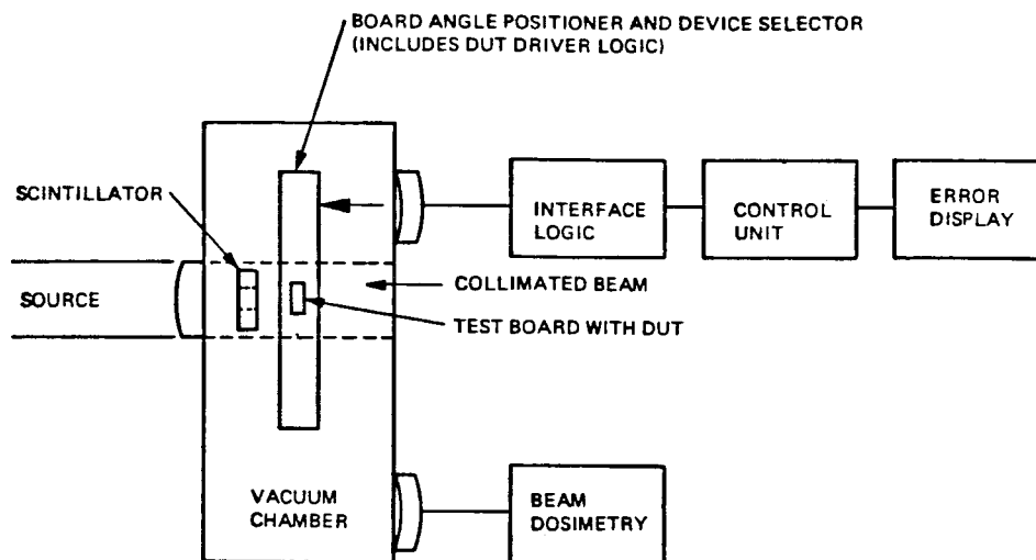
NOTE 1—See also Fig. 2 and Fig. 3. FIG. 1 Typical Schematic Overview of SEP Test
