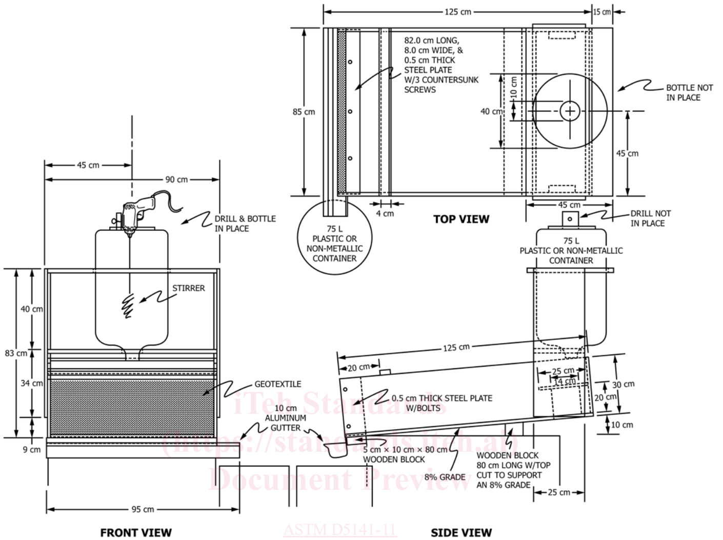
NOTE 1—Sides and bottom of flume can be constructed of 2-cm thick marine grade plywood. https://standards.ansi.org/astm-d5141-11 FIG. 1 Flume (For Vertical SRDs)
