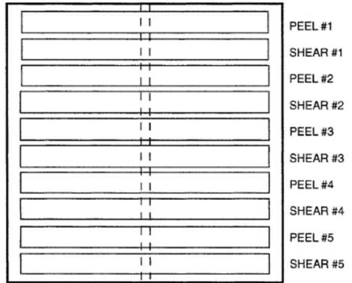
FIG. 1 Specimen configuration of seam sample.
