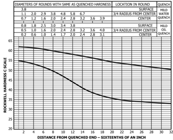
FIG. 16 Limits for Hardenability Band 4142 H
