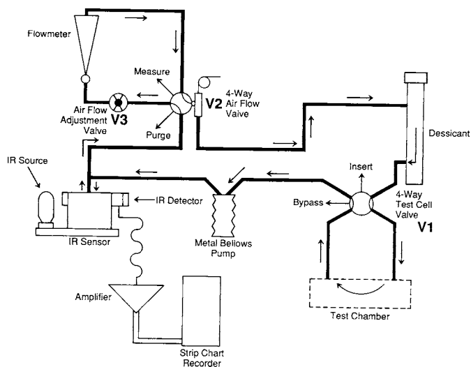
FIG. 1 Measuring System
