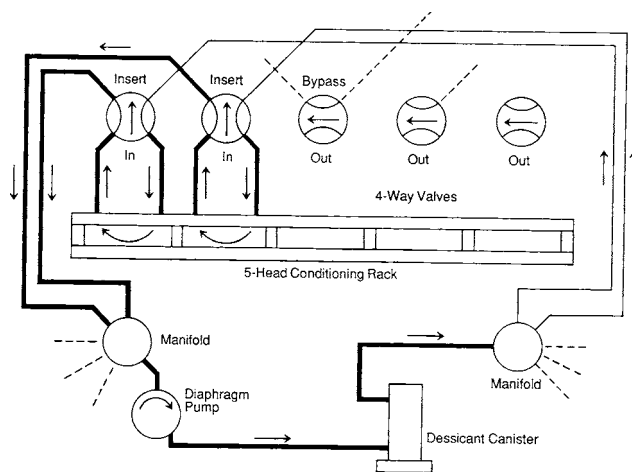
FIG. 2 Conditioning System
