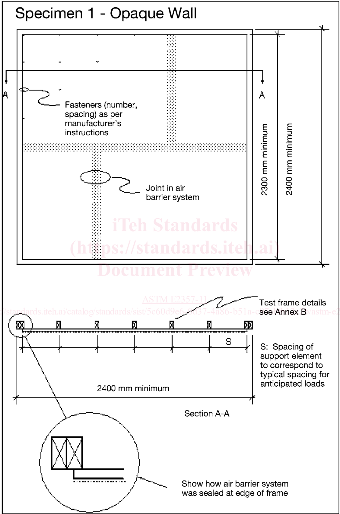
FIG. A1.1 Specimen 1—Opaque Wall
