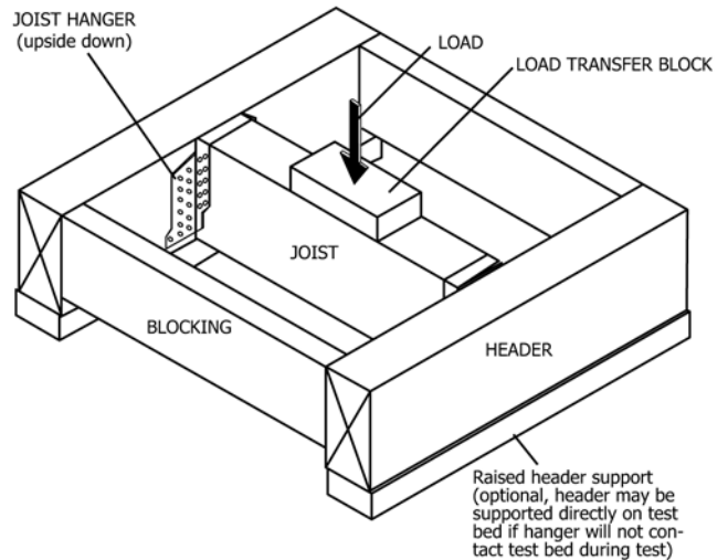
FIG. 2 Typical Uplift Test Setup
