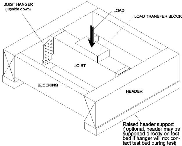
FIG. 2 Typical Uplift Test Setup
