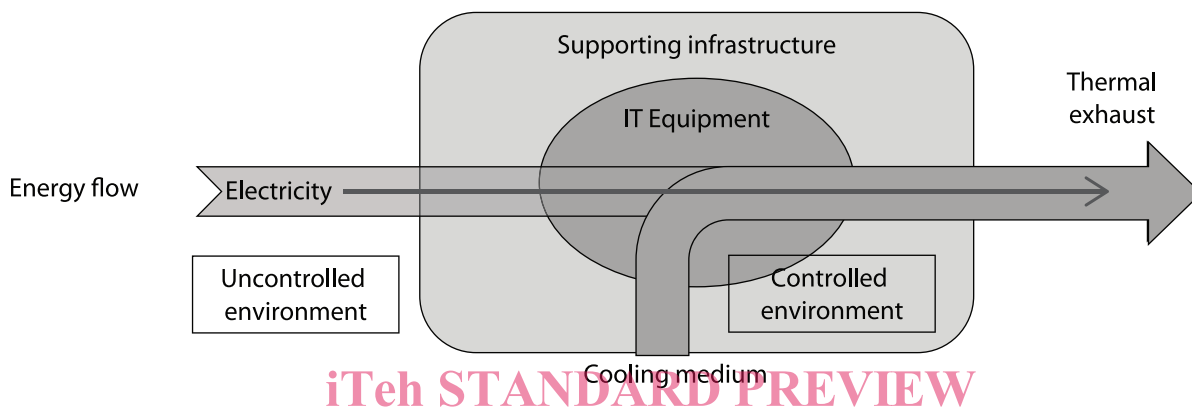
Figure 2 — Logical representation of environmental control of data centre spaces
