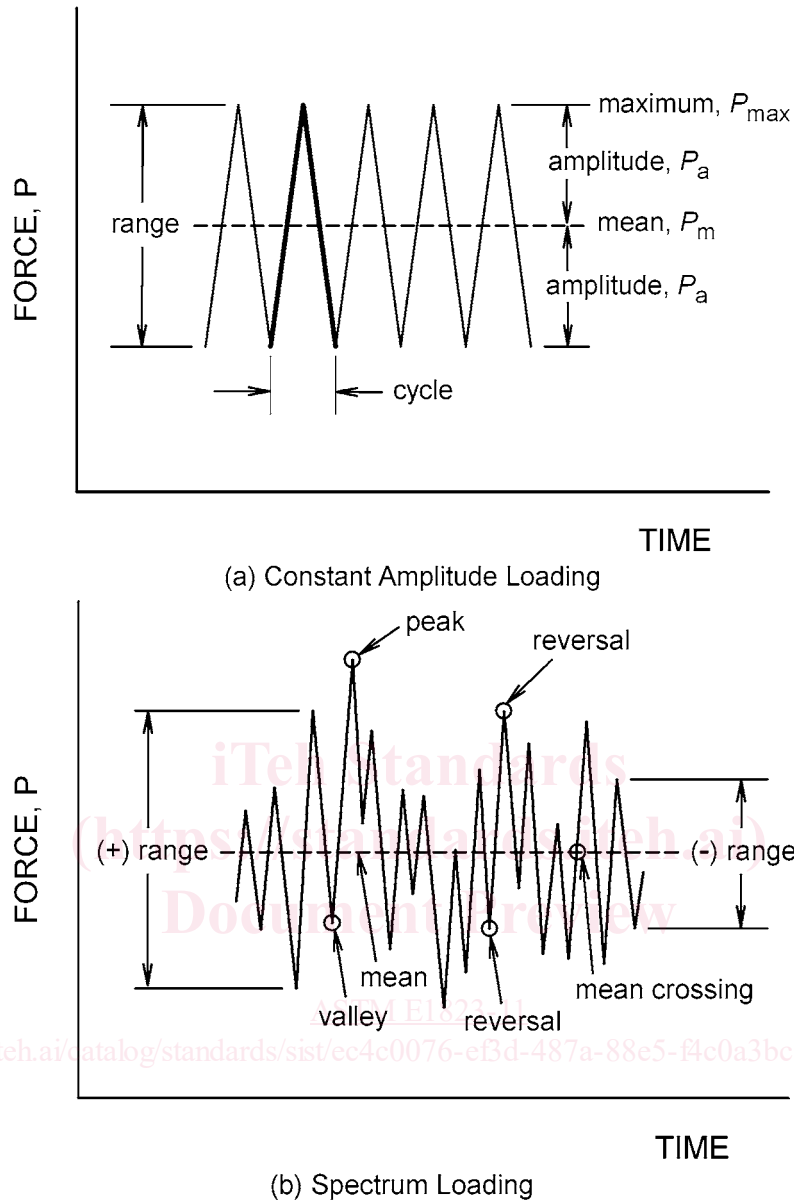
FIG. 3.4 Fatigue Loading Basic Terms
