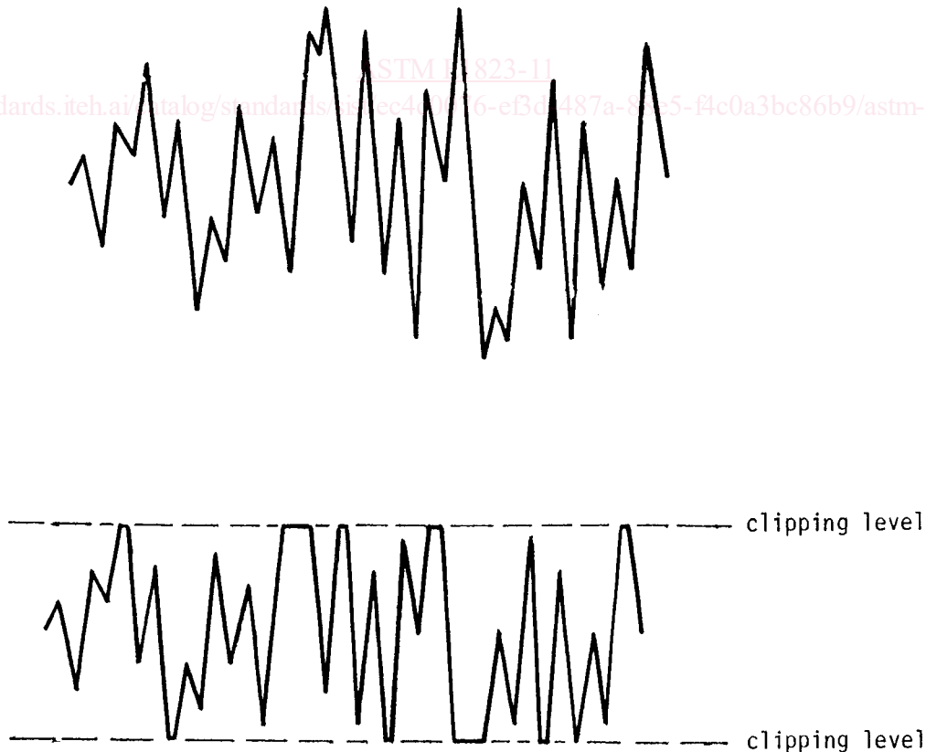
FIG.-2_3 Clipping of Fatigue Spectrum Loading
