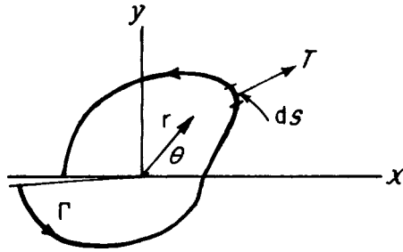
FIG.-7_2 J-Integral Contour and Symbolism
