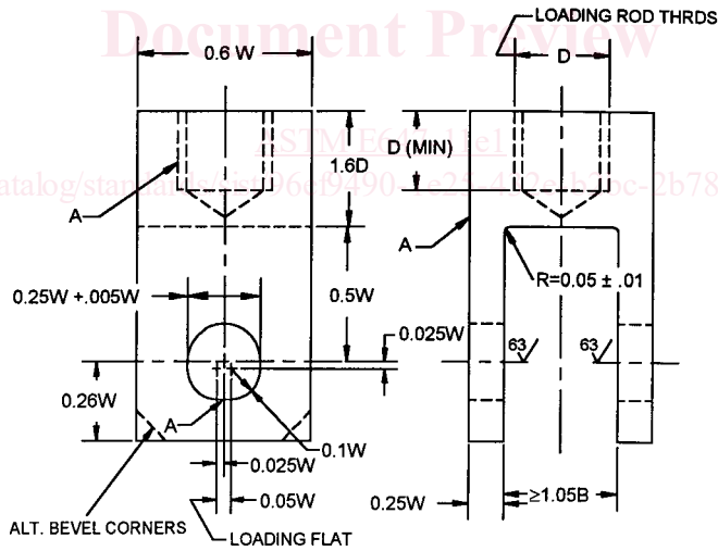
FIG. A1.2 Clevis and Pin Assembly for Gripping C(T) Specimens
