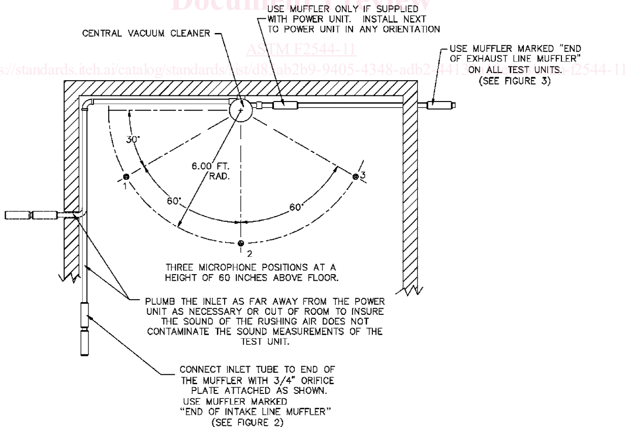
FIG. 1 Sound Test Layout
