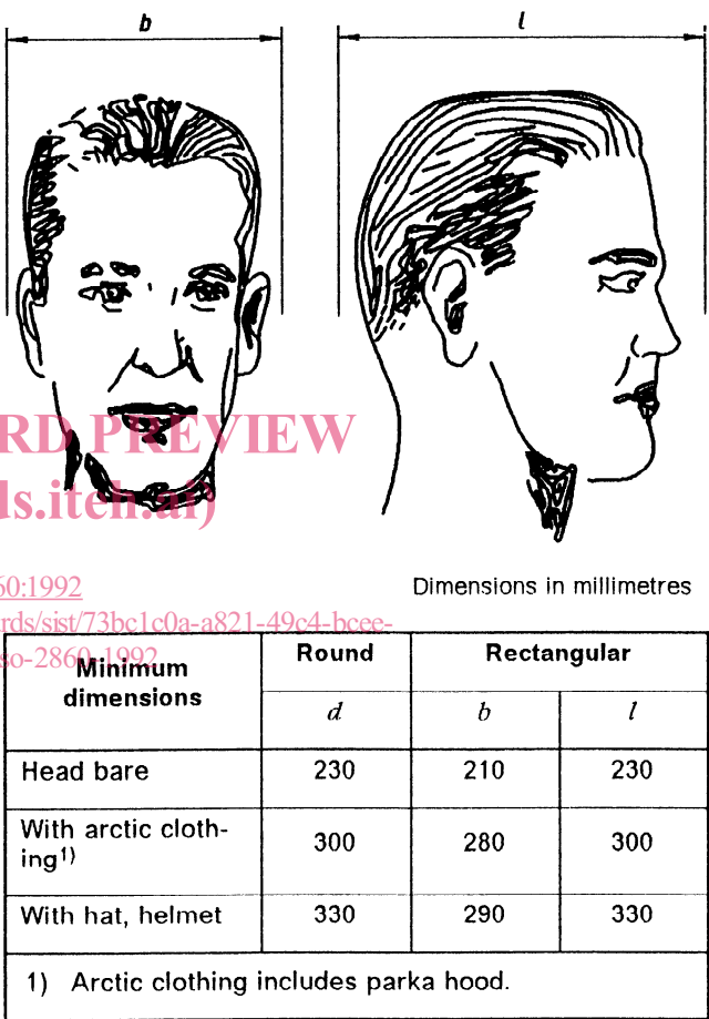
Figure 2 — Minimum dimensions for head access, 95th percentile
