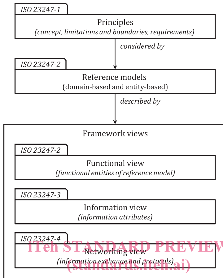
ISO 23247-4:2021 Figure 1 — ISO 23247 series structure https://standards.iso.org/standards.html?csd=2-469b-adb3-846ea5b64d5/iso-23247-4-2021
