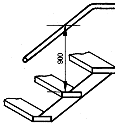
Figure 4 — Main courante
