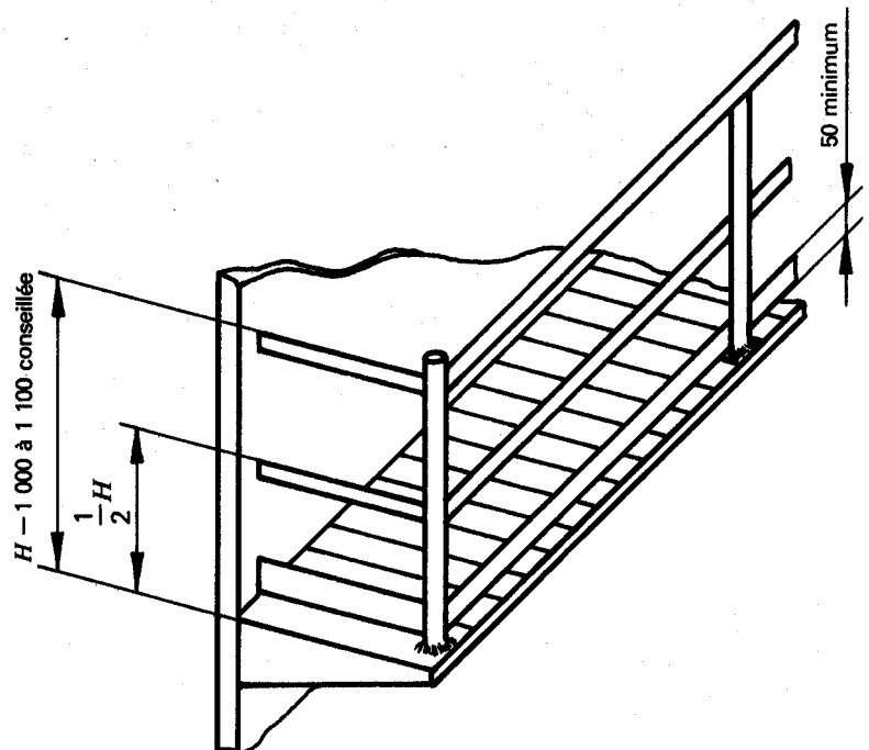
Figure 6 — Garde-corps
