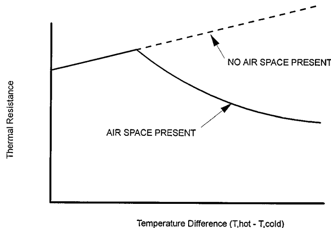
NOTE 1—A constant hot-side temperature ( T_{hot} ) is used for both tests and the temperature difference increases as the cold side temperature ( T_{cold} ) is decreased. See 5.1.6 for requirements on size of air space.
