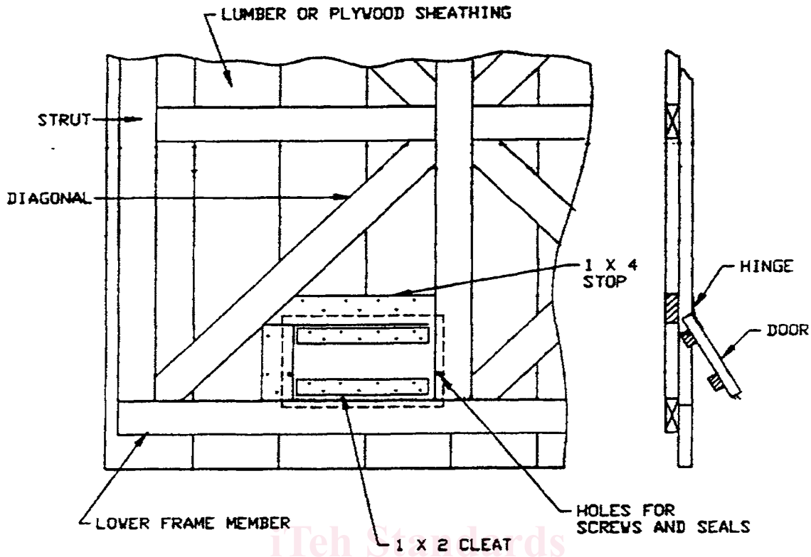
NOTE—All dimensions in inches. FIG. 5 Inspection Door (Inside View)
