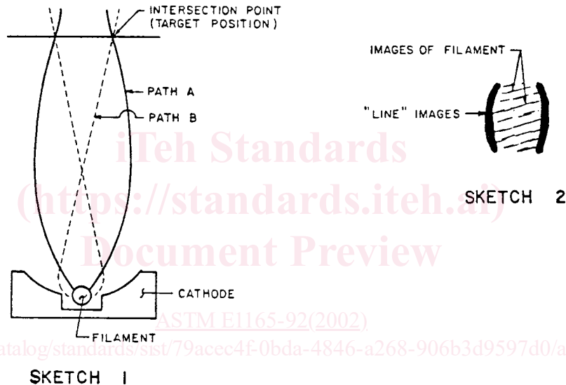
FIG. 2 Actual/Effective Focal Spot
