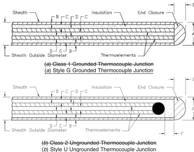
FIG. 3 Sheathed Thermocouple Assembly
