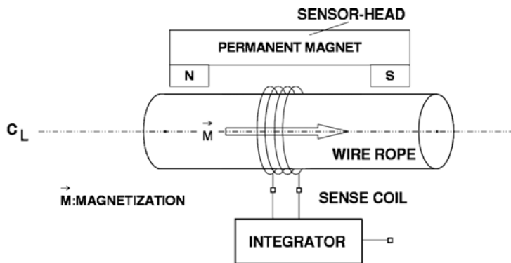
FIG. 2 1 Schematic Representation of a Permanent Magnet Equipped Sensor-Head Using a Sense Coil to Measure the Loss of Metallic Cross-Sectional Area
