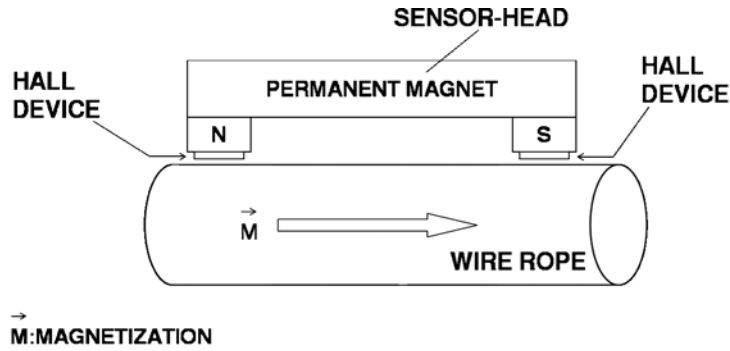
FIG.-3_2 Schematic Representation of a Permanent Magnet Equipped Sensor-Head Using Hall Devices to Measure the Loss of Metallic Cross-Sectional Area
