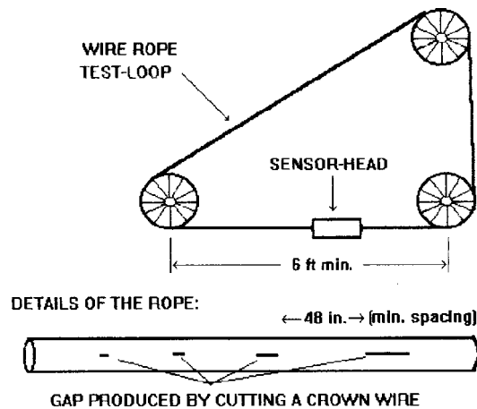
FIG.-5_4 Example of a Wire Rope Reference Standard
