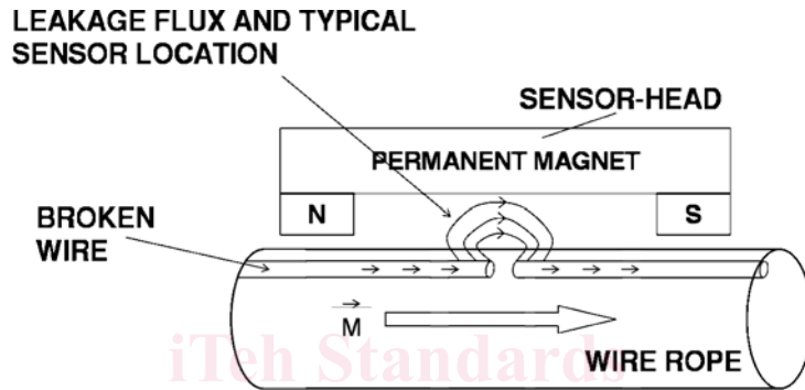
FIG.-4_3 Illustration of the Leakage Flux Produced by a Broken Wire
