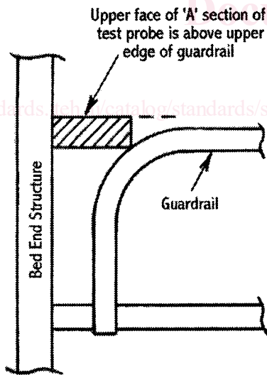
FIG. 7 (a) Partially Bounded Opening (Conforms to Requirement)
