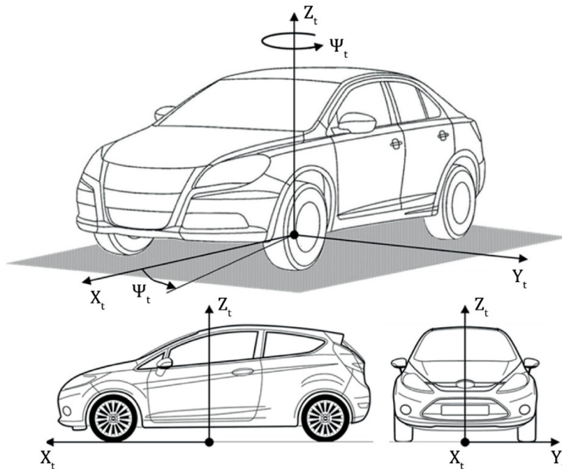
Figure 3 — Vehicle reference coordinate system (Source: ISO 19206-3:2021, Figure 2)
