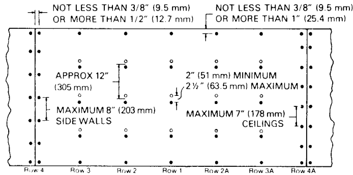
FIG. 3 Double Nailing
