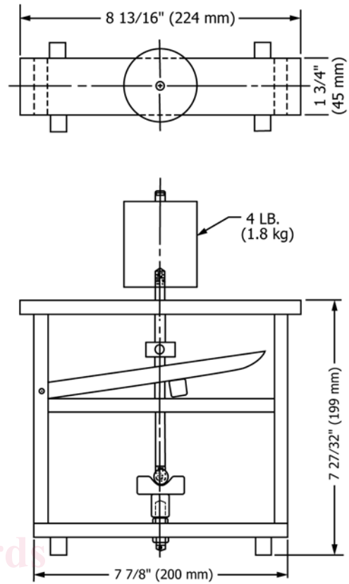
FIG. 2 Curved Electrode and Holder
