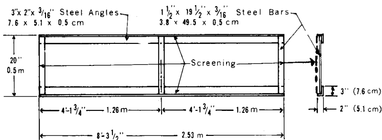
FIG. 6 Steel Frame for Loose Fill Insulation Materials
