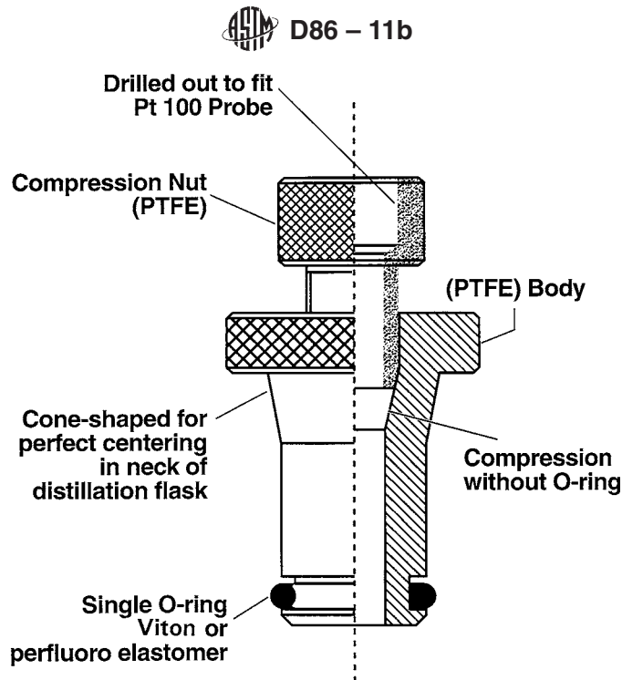
FIG. 4 Example of Centering Device Designs for Straight-Bore Neck Flasks
