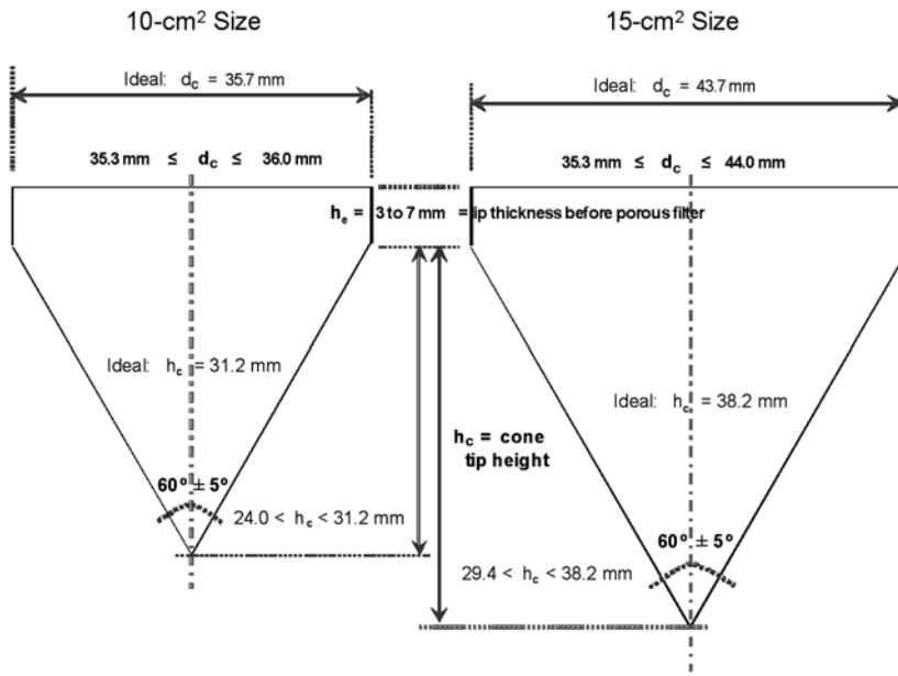
FIG. 2 Manufacturing and Operating Tolerances of Cones (35)
