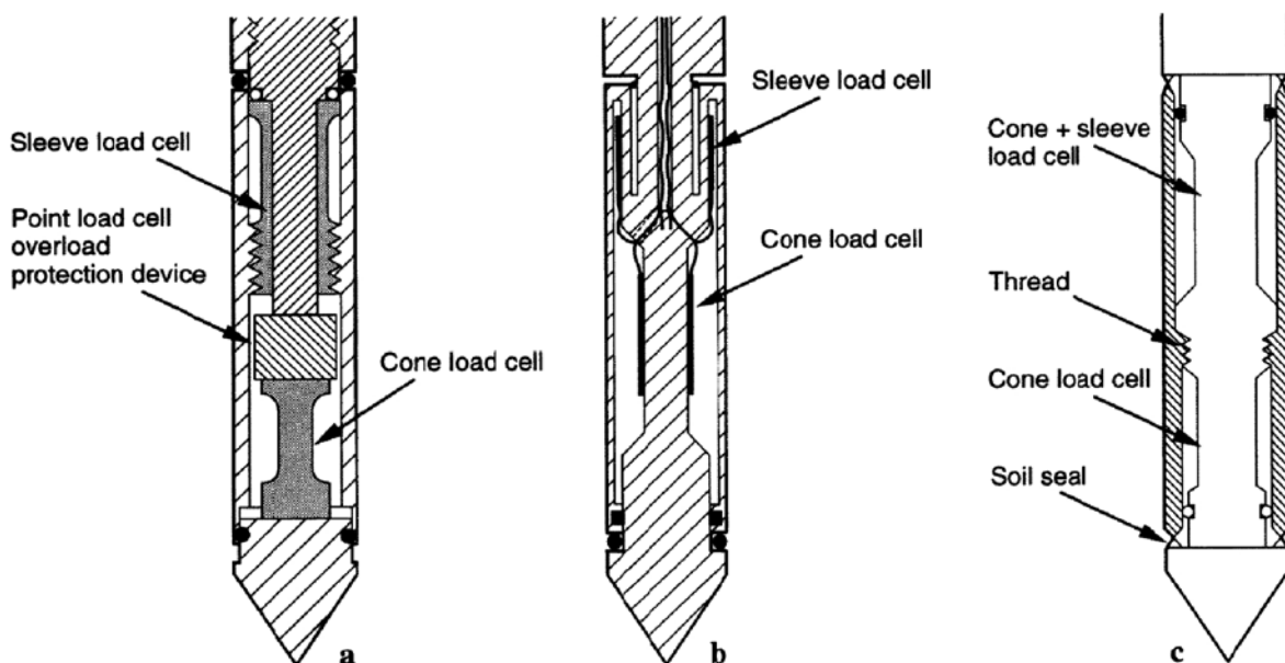
FIG. 1 Common Configurations for Electric Friction-Cone Penetrometers (24) Showing: (a) Compression-type Tip and Sleeve Load Cells, (b) Tension-type Sleeve Design, and (c) Subtraction-type Penetrometer
